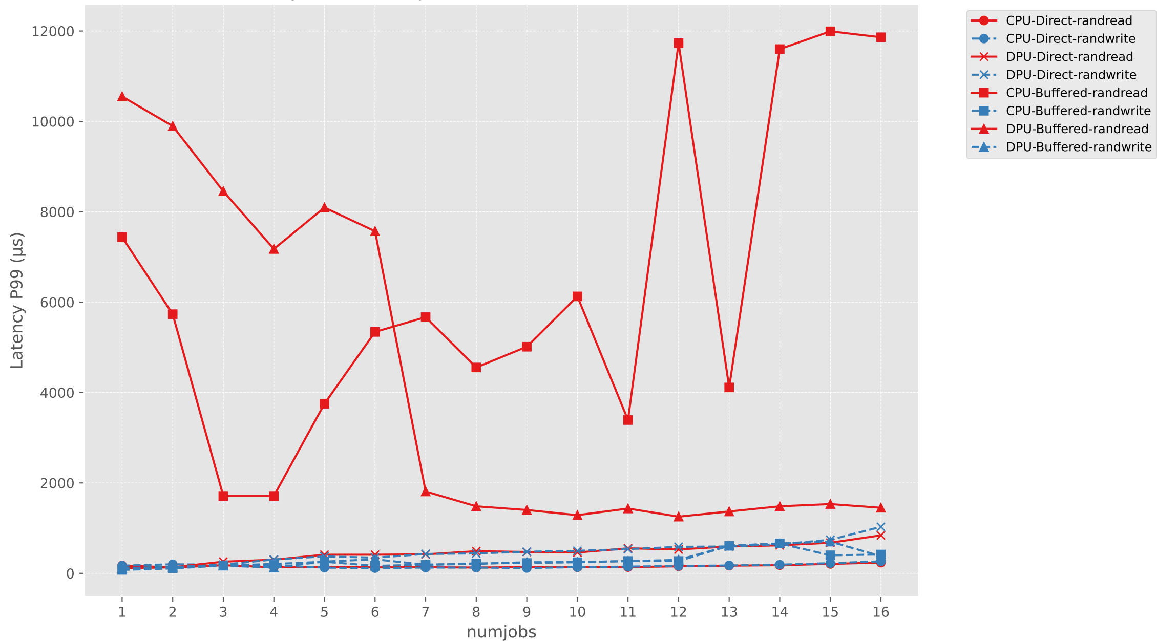
Latency P99 vs numjobs (CPU vs DPU, Direct vs Buffered)
